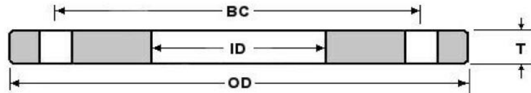
AWWA Slip On Ring Flange
