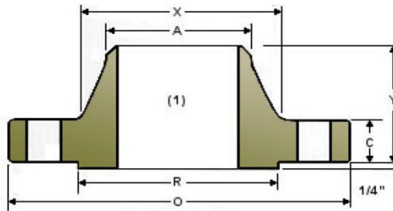
WELDING NECK
