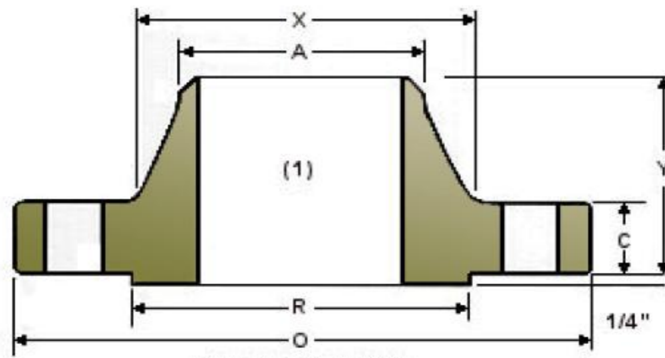
WELDING NECK
