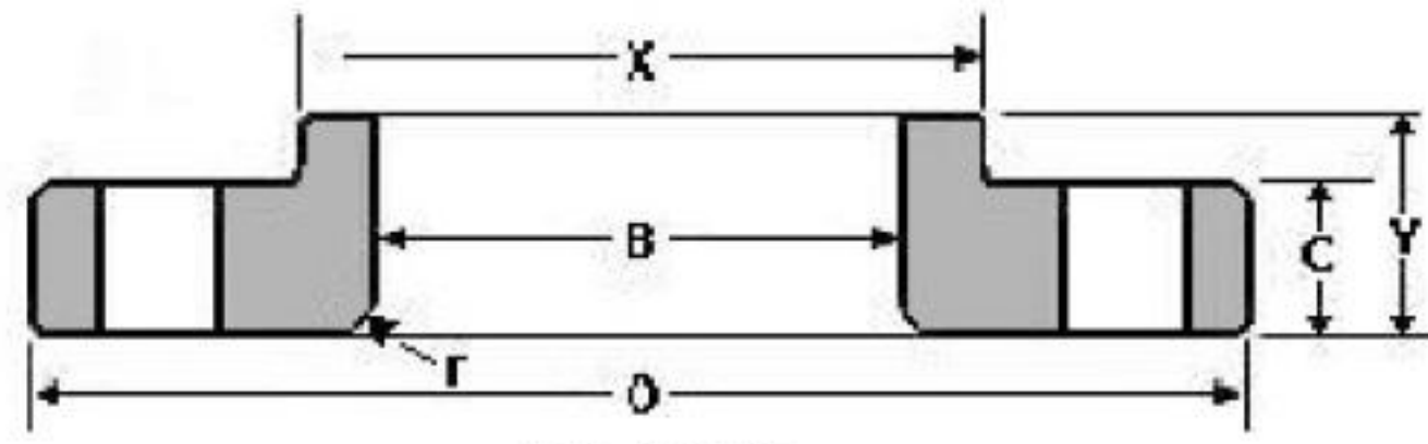
LAP JOINT
