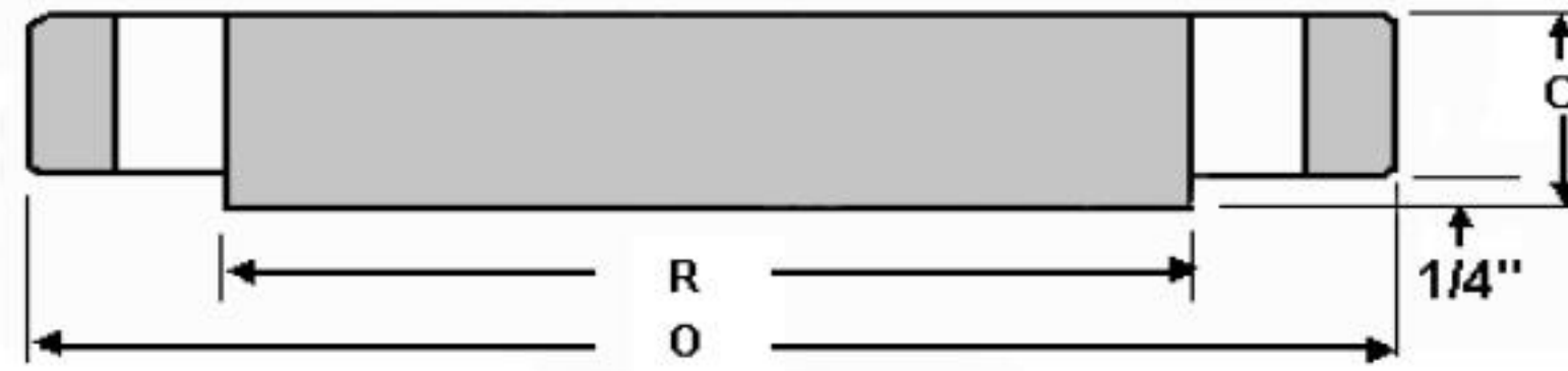
BLIND FLANGE
