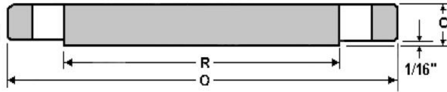
BLIND FLANGE
