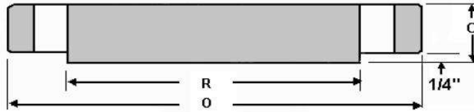
BLIND FLANGE
