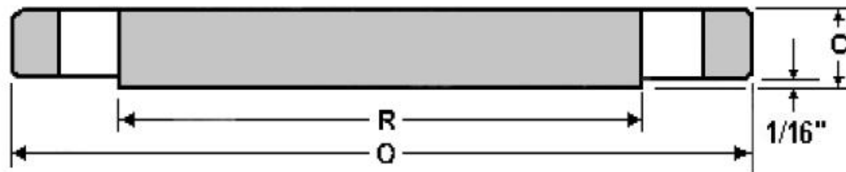
BLIND FLANGE
